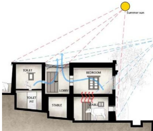
Figure 4: Typical section [11]
