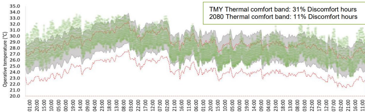
Figure 11: OT of the workstation room with rammed earth wall (with insulation), the grey area shows the future weather, and the two red lines show the TMY adaptive thermal comfort band according to NBC
