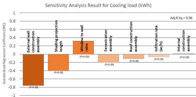
Figure 10 - SRC for Cooling load,
