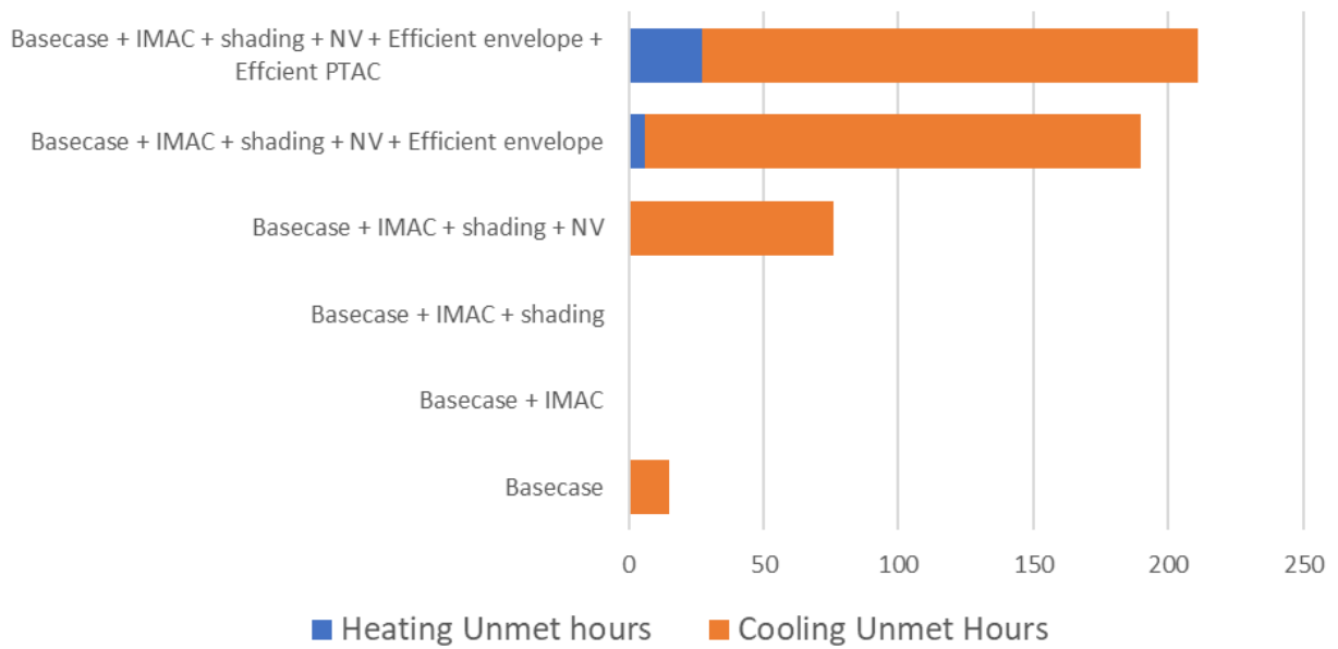
Figure 14 - Unmet hours
